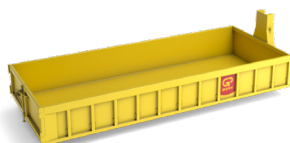
12 m 3 open container L 6,0m x B 2,5m x H 1,0m
